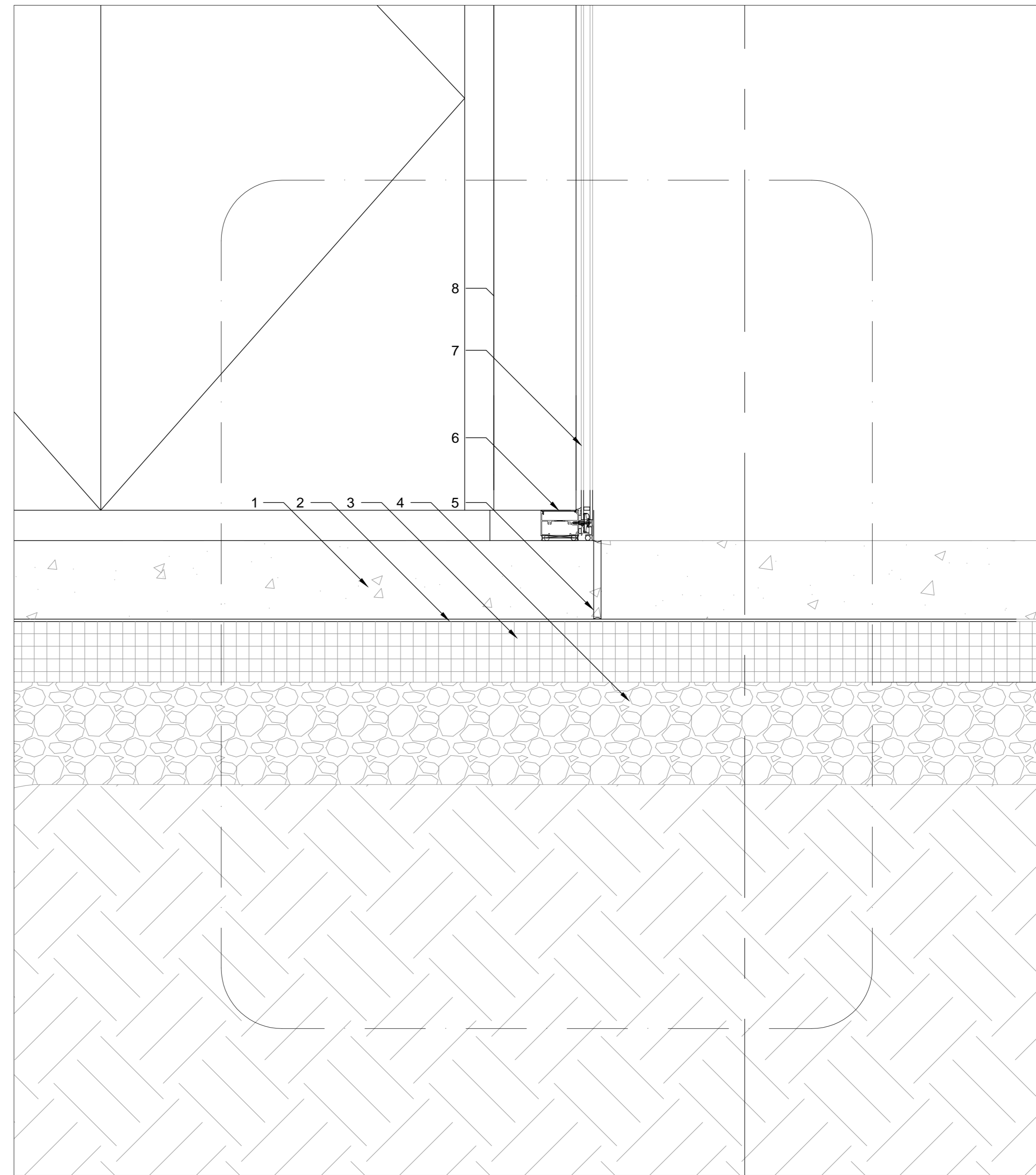
2 Detail A352 Scale 1-1/2" = 1'-0"
