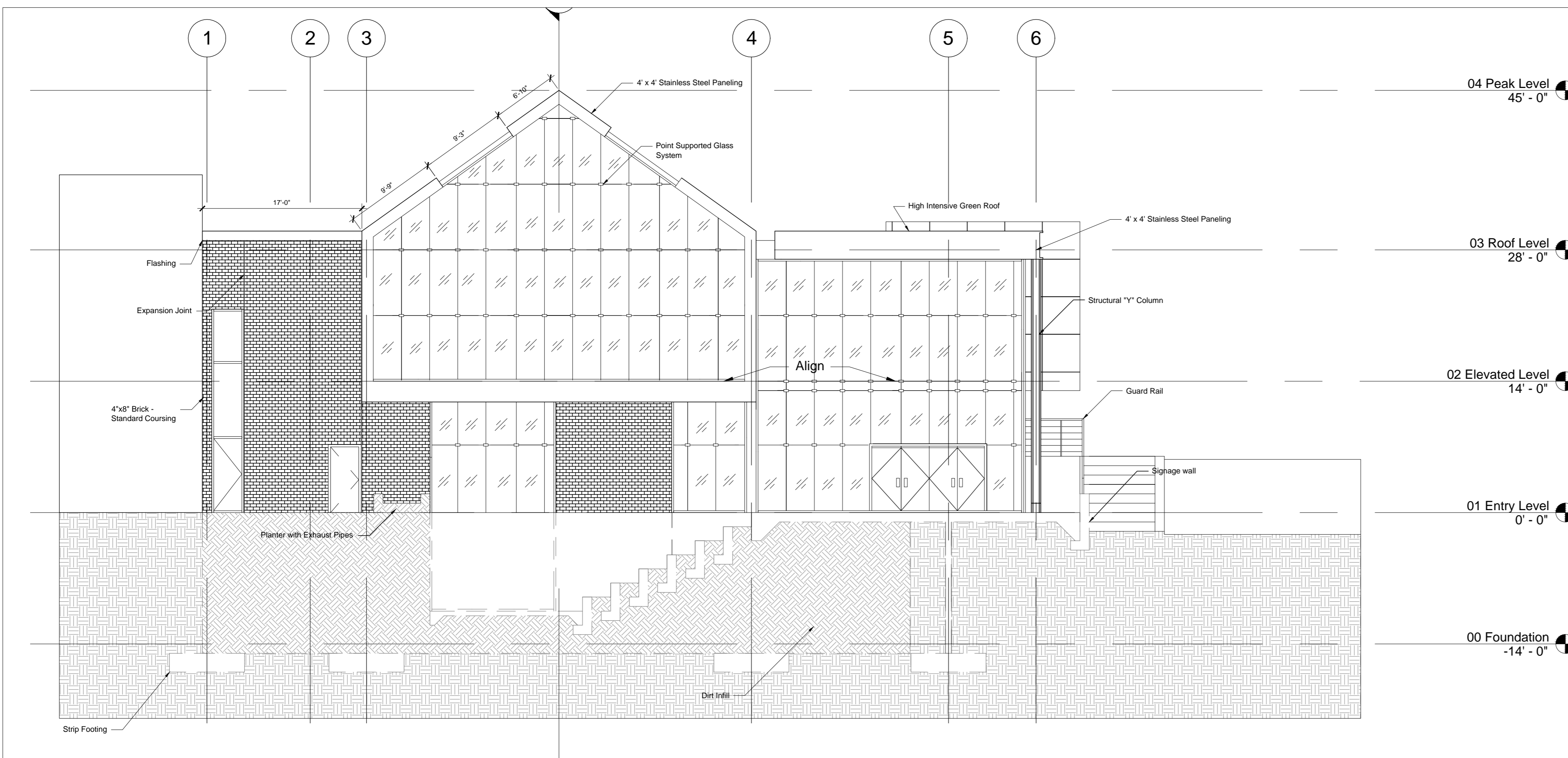
2 East Elevation A200 Scale 1/8" = 1'-0"
