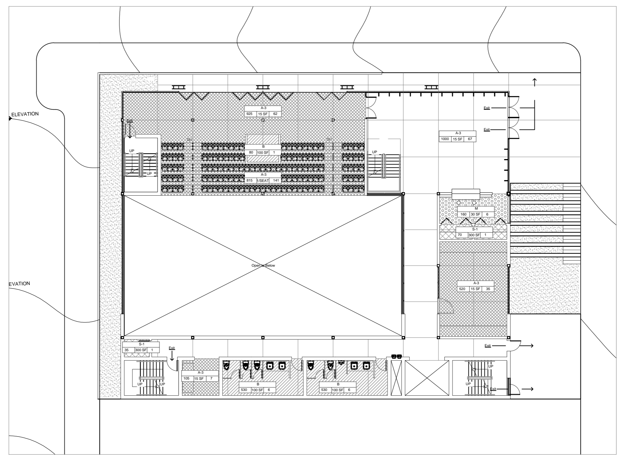
2 01 Plan Life Safety LS100 Scale 1/8" = 1'-0"
