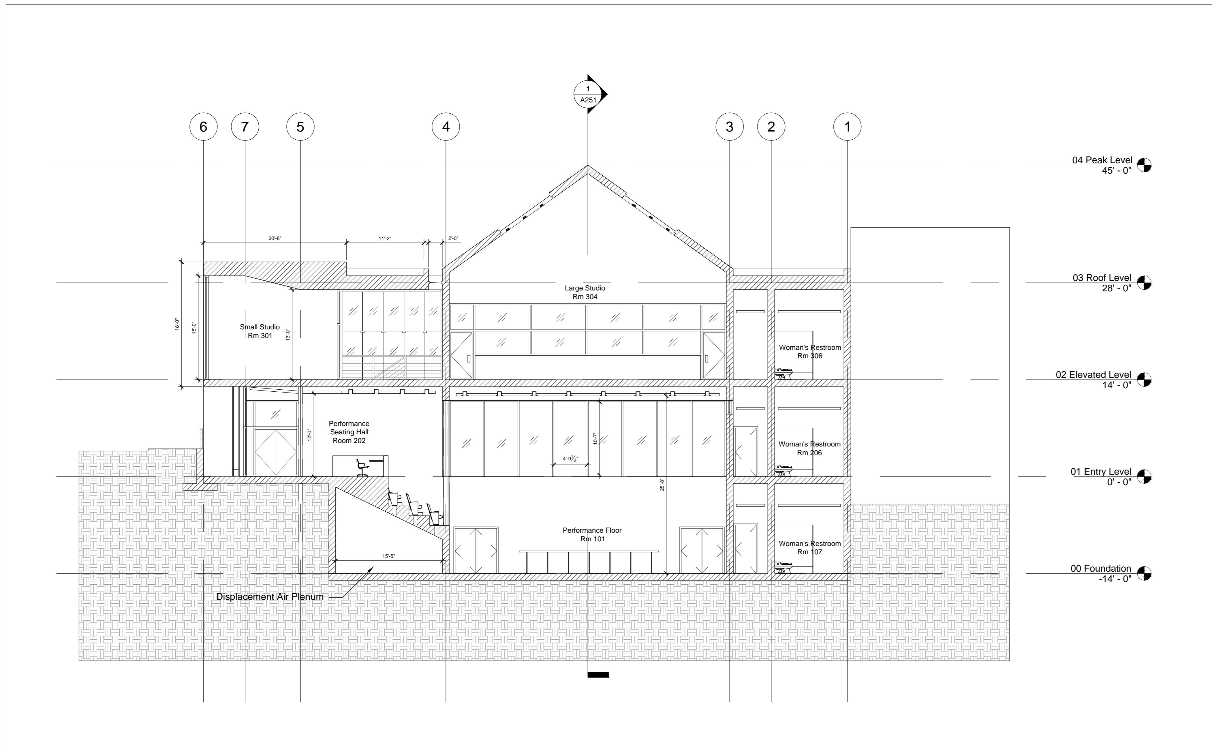
1 Transverse Section A250 Scale 1/8" = 1'-0"
