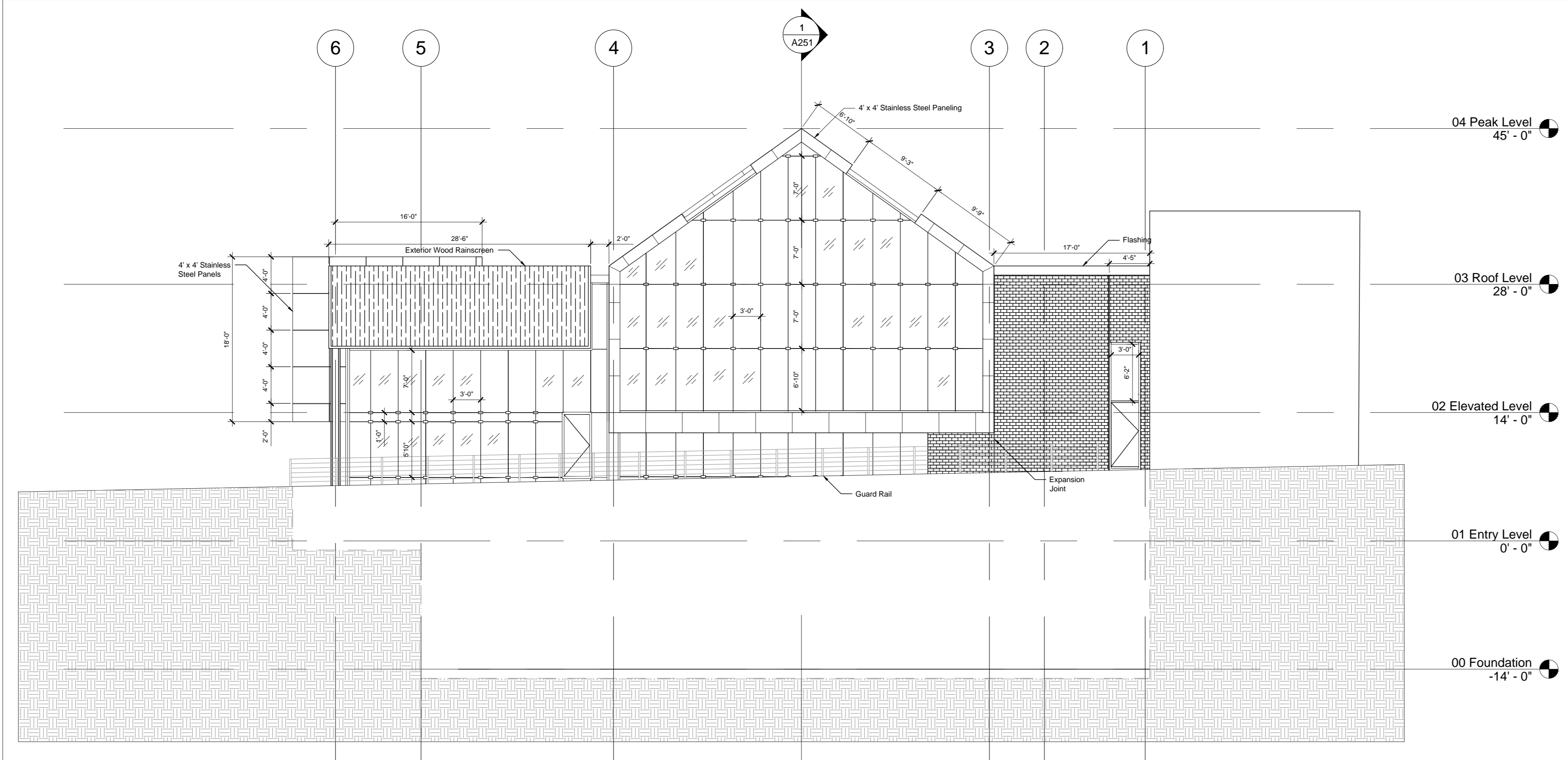
1 West Elevation A200 Scale 1/8" = 1'-0"
