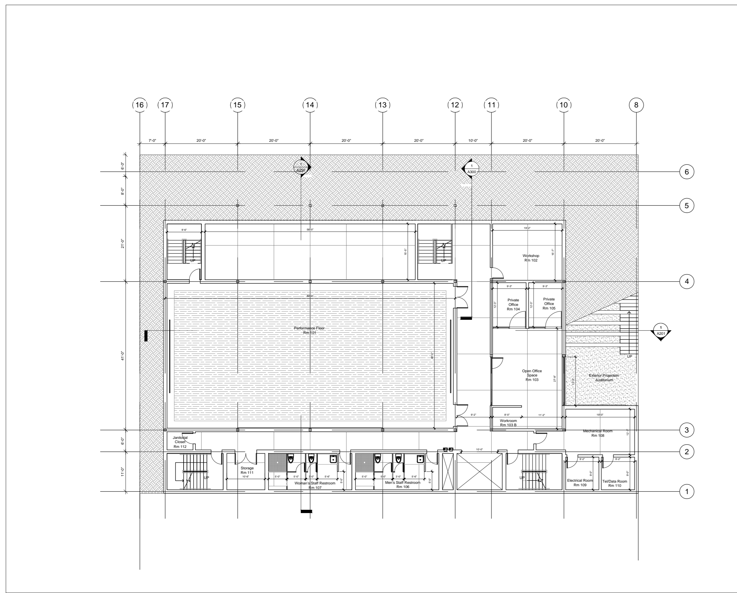
1 00 Mechanical Plan M100 Scale 1/8" = 1'-0"
