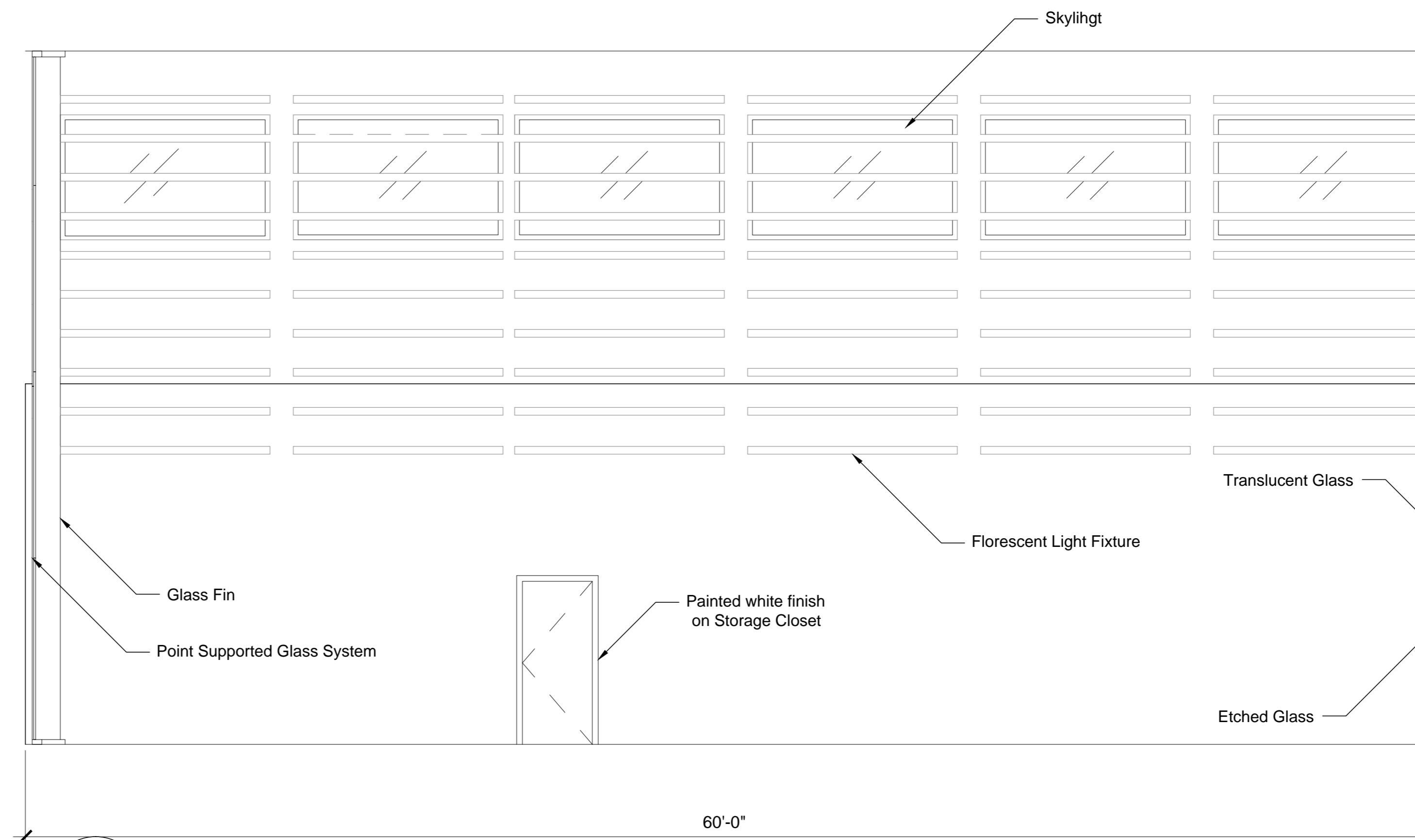
2 South Interior Elevation A601 Scale 1/4" = 1'-0"
