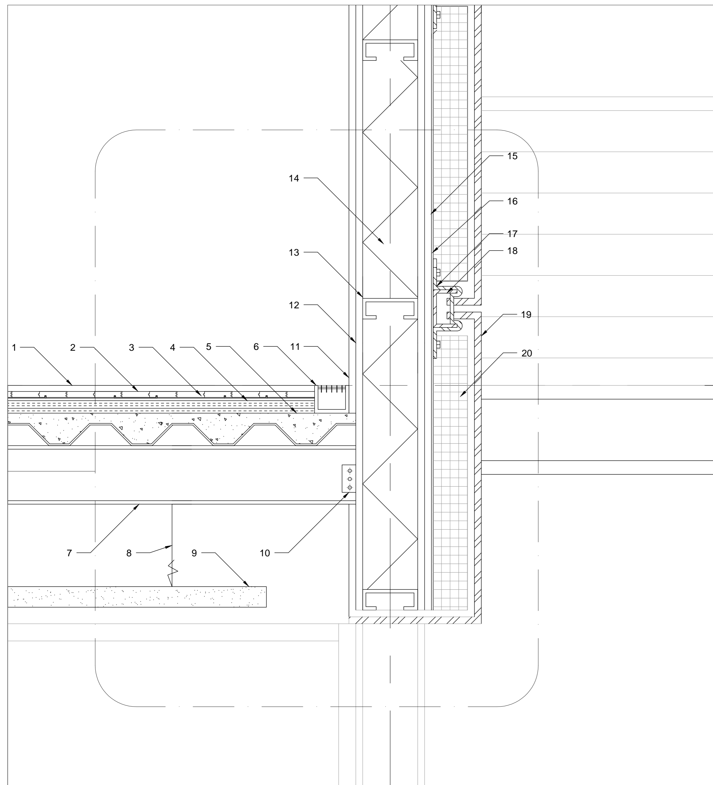
1 Detail A351 Scale 1-1/2" = 1'-0"
