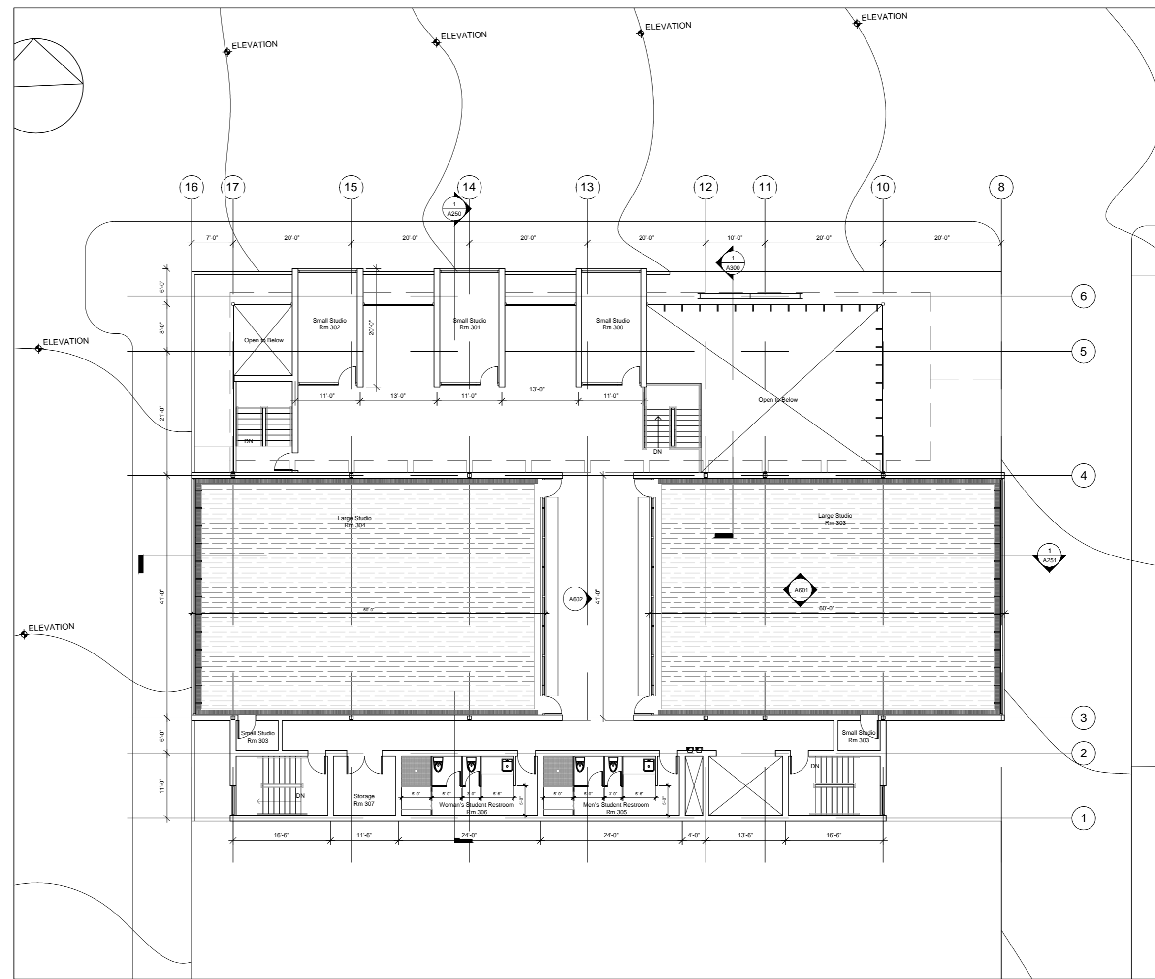
2 01 Mechanical Plan M100 Scale 1/8" = 1'-0"
