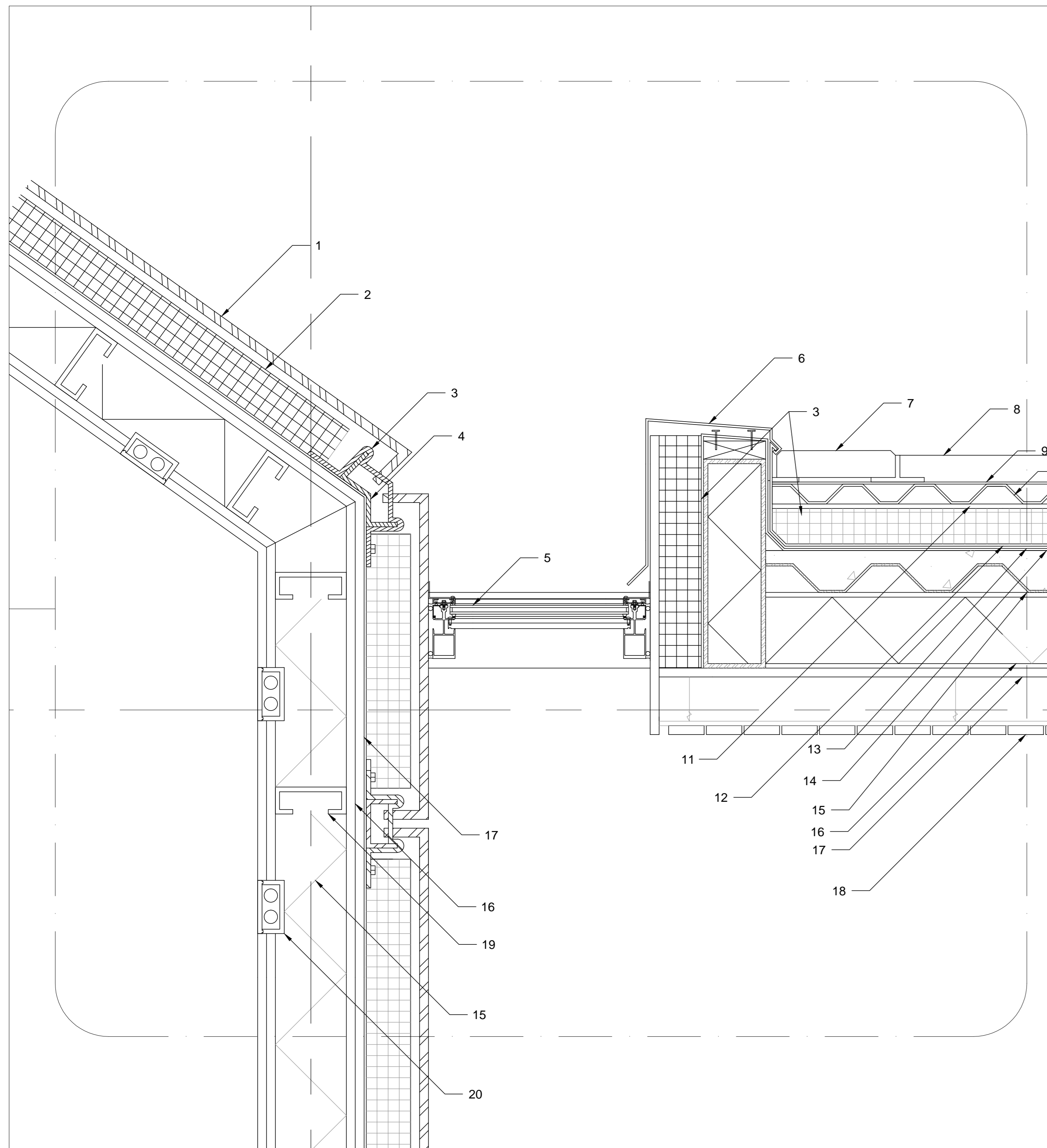
1 Detail A350 Scale 1-1/2" = 1'-0"
