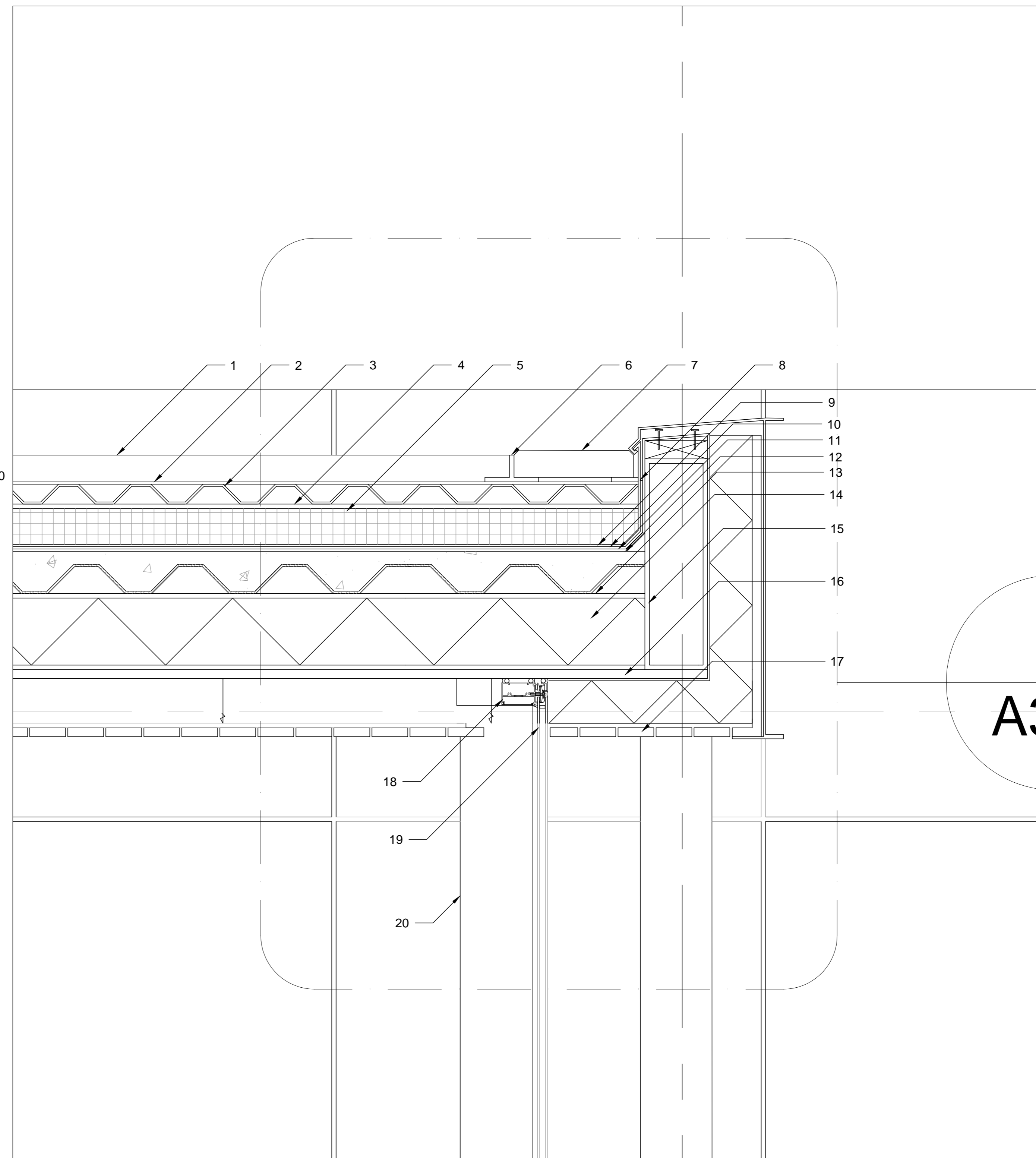
2 Detail A350 Scale 1-1/2" = 1'-0"
