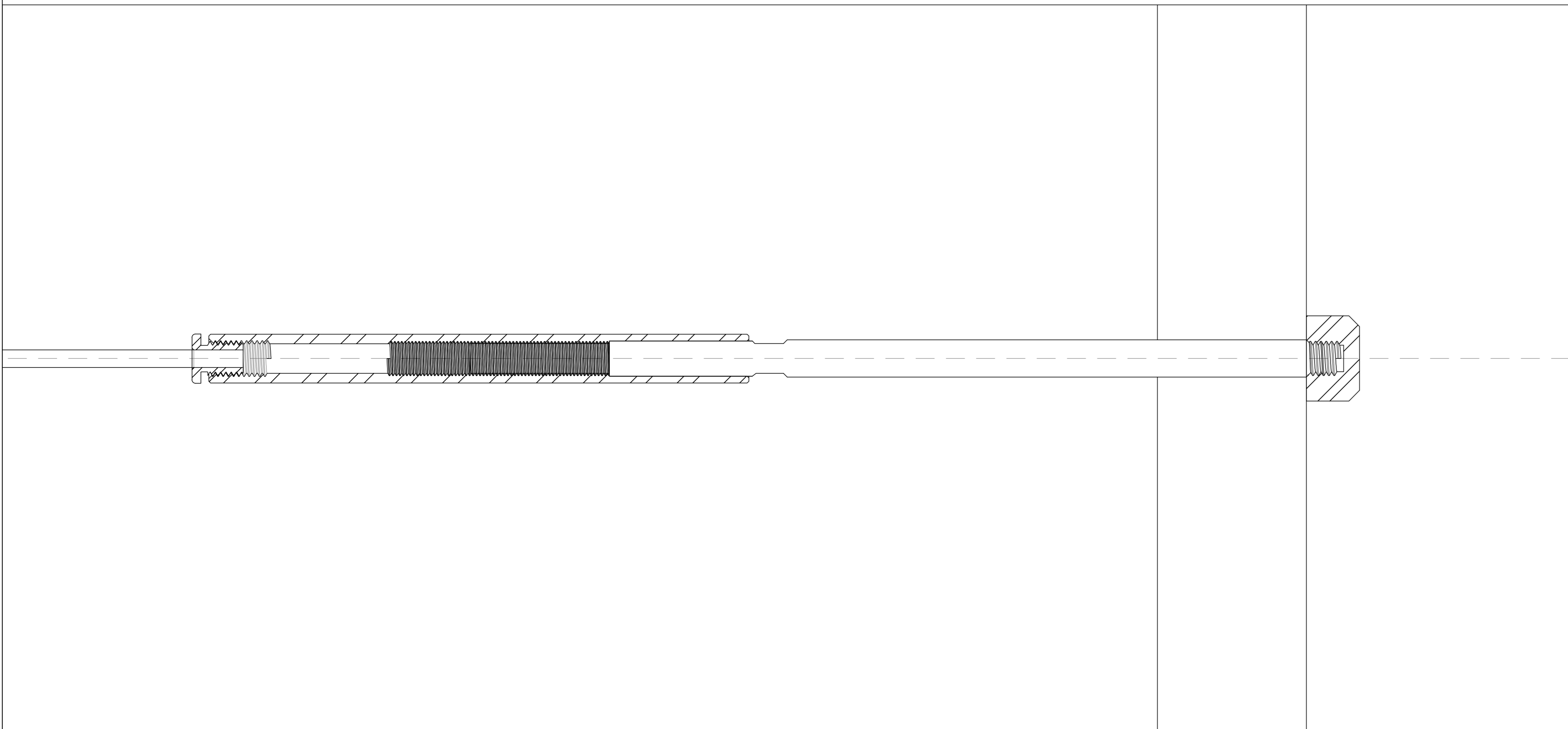
2 Railing Detail A353 Scale 2:1
