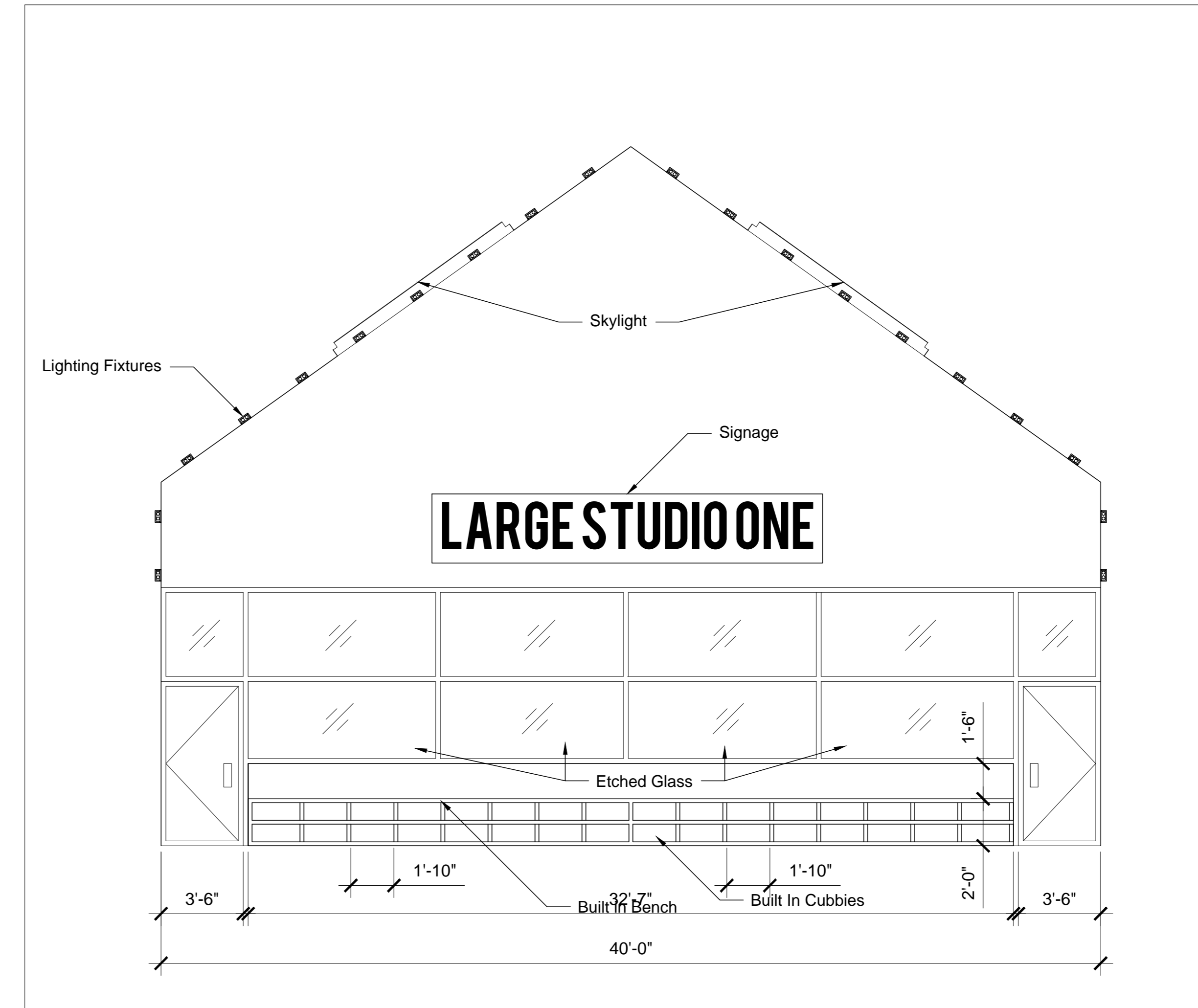
2 West Interior Elevation A602 Scale 1/4" = 1'-0"
