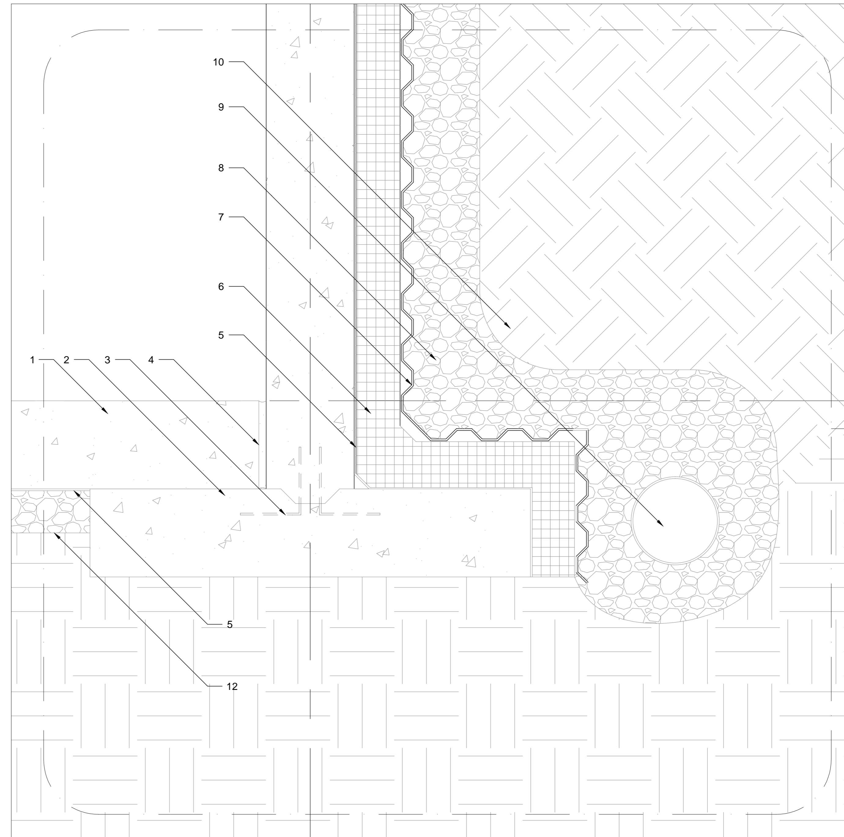
2 Detail A351 Scale 1-1/2" = 1'-0"
