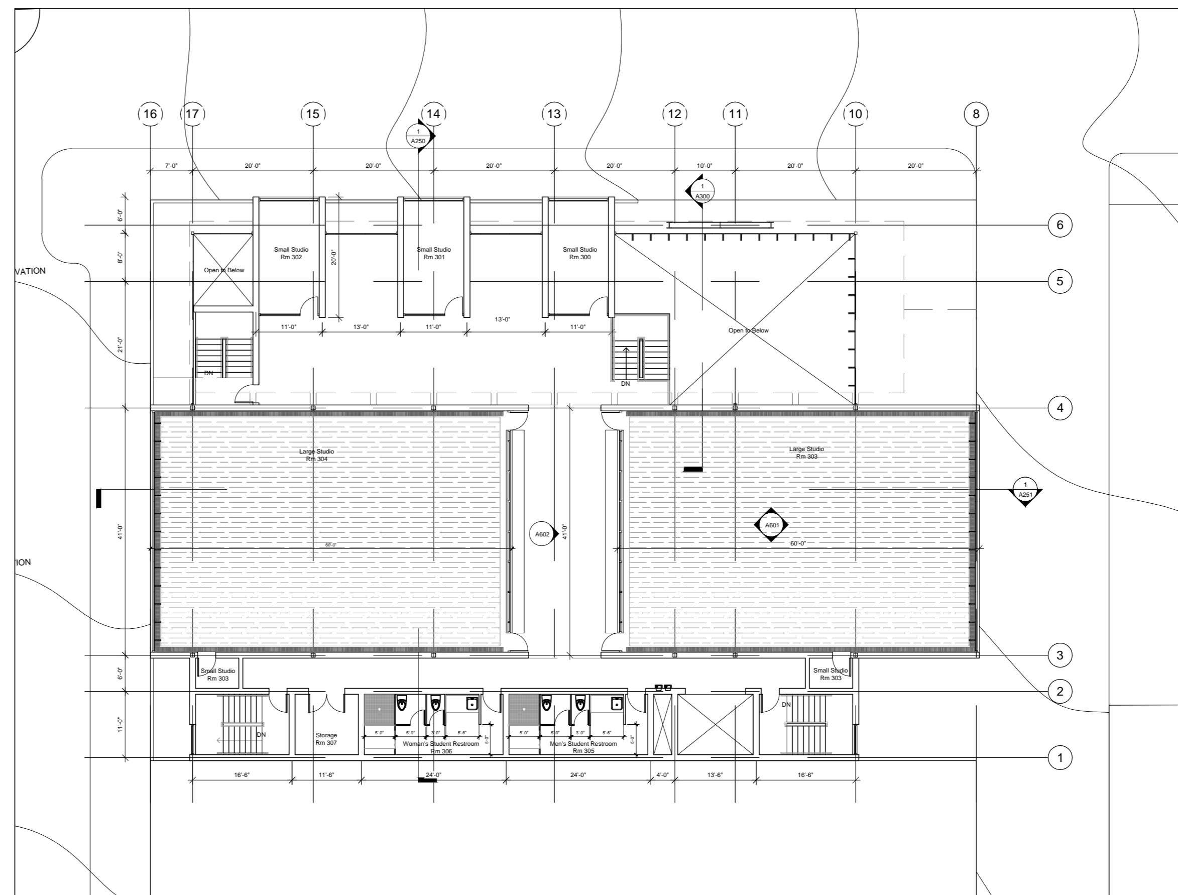
3 02 Mechanical Plan M100 Scale 1/8" = 1'-0"
