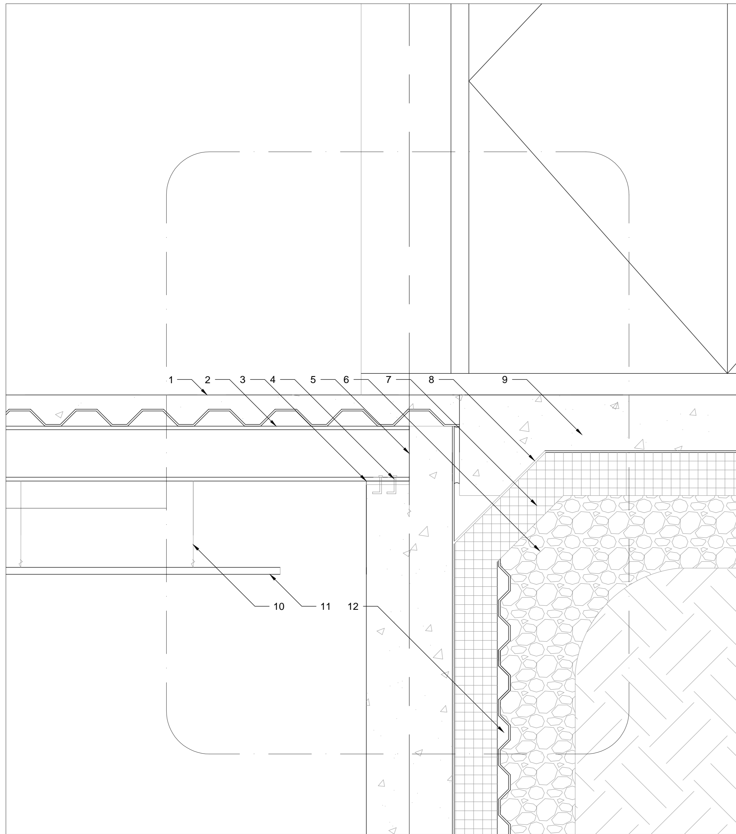
1 Detail A352 Scale 1-1/2" = 1'-0"
