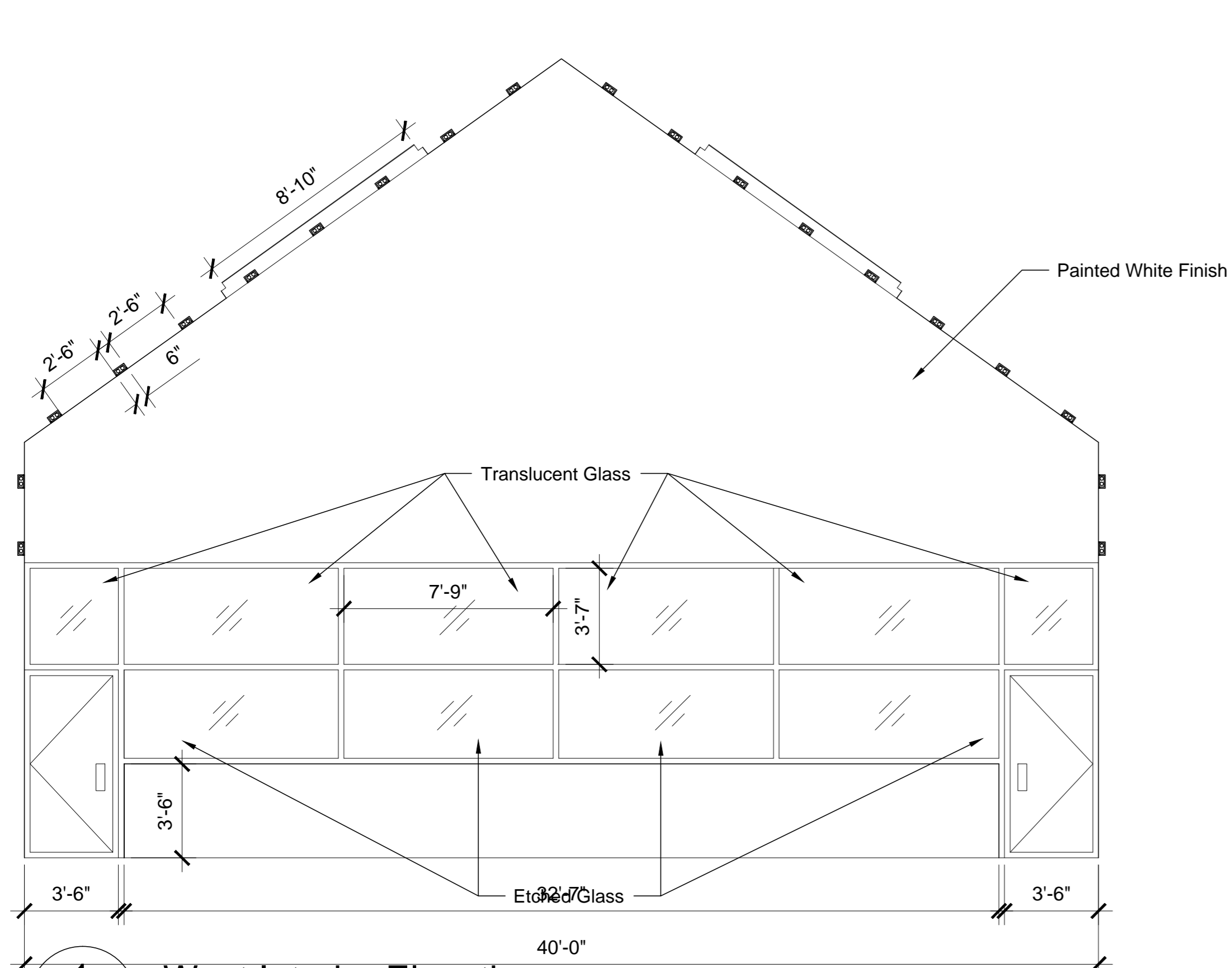
1 West Interior Elevation A601 Scale 1/4" = 1'-0"
